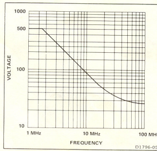
Fig. 3. Voltage vs. frequency derating.
