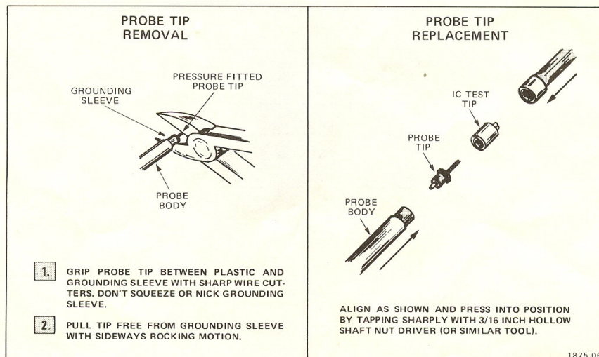
Fig. 4. Probe tip removal and replacement.
